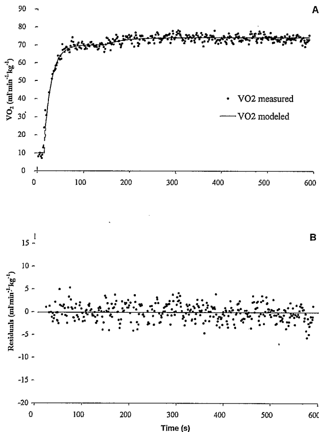
FIGURE 1—Example for subject 1: fit of the modeled \text{O}_2 uptake in the heavy constant-rate exercise (A) and distribution of the residual sum of squares (B).
